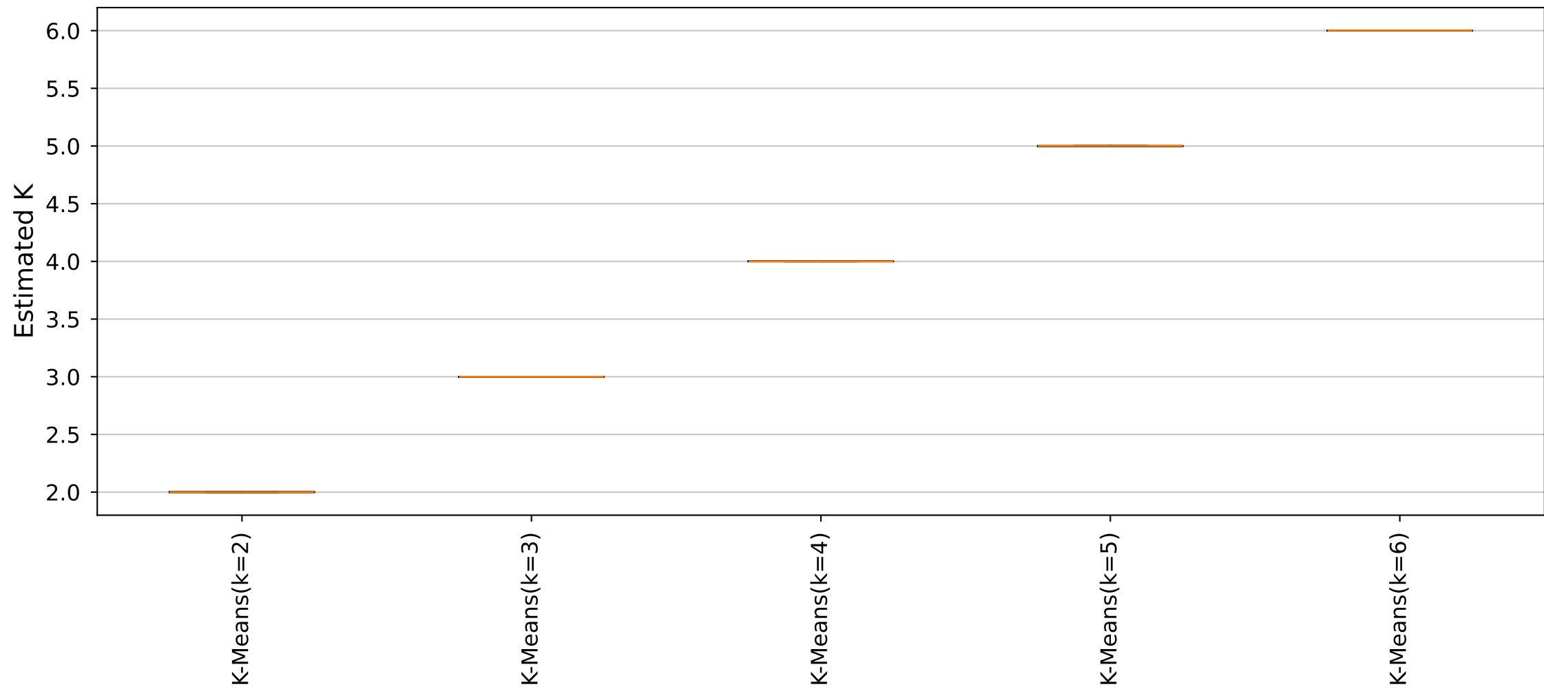
YARA Rules Estimated K Distribution (Cluster25_Size6 dataset)
